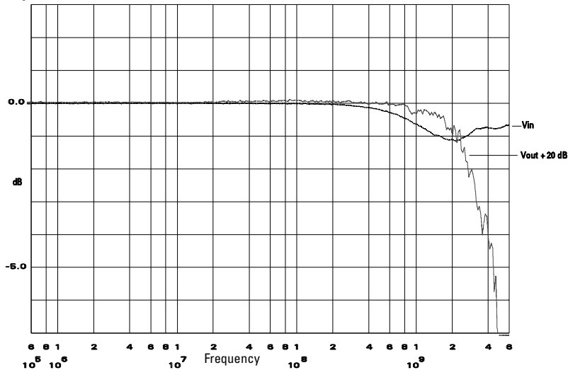
Graph of Vin to Probe and Vout of Probe with 25 Ω Source
